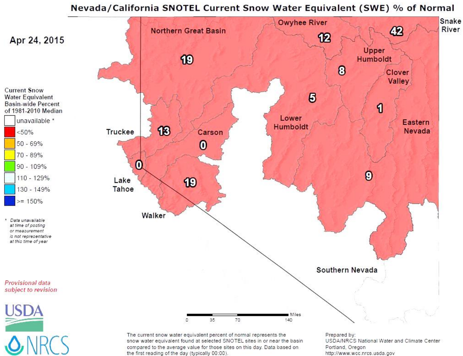
Figure 3. Percent of normal snow water equivalent (SWE) for the state of Nevada and portions of California. Data was generated on 24 April 2015 from the USDA funded website: http://www.wcc.nrcs.usda.gov .
